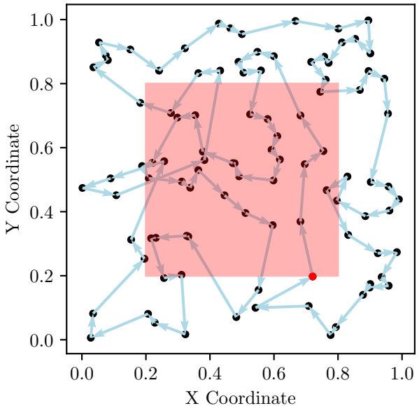
TSP Route, Cost: 9.88
