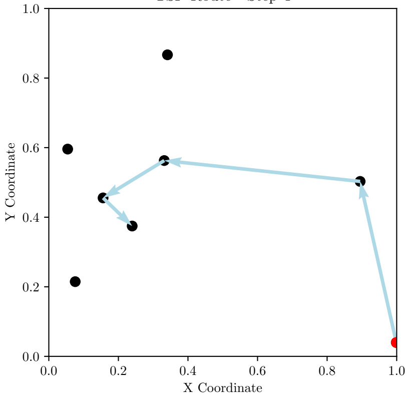
TSP Route - Step 4
