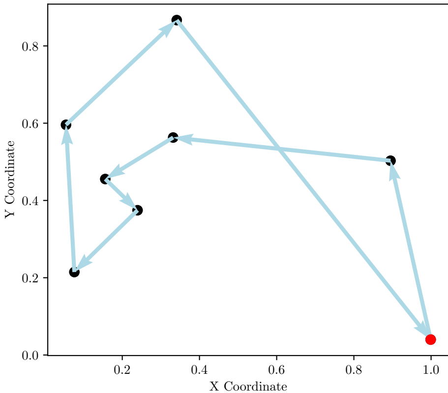
TSP Route, Cost: 3.43
