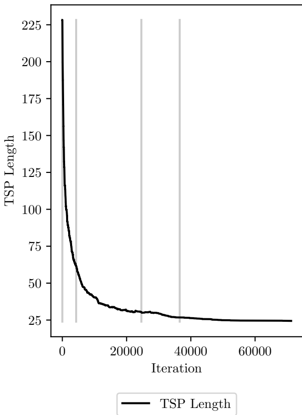
TSP cost evolution, final cost: 24.42
