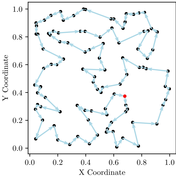
TSP Route, Cost: 8.41
