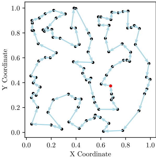
TSP Route, Cost: 8.09
