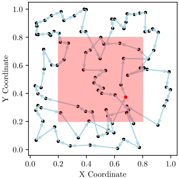
TSP Route, Cost: 9.90
