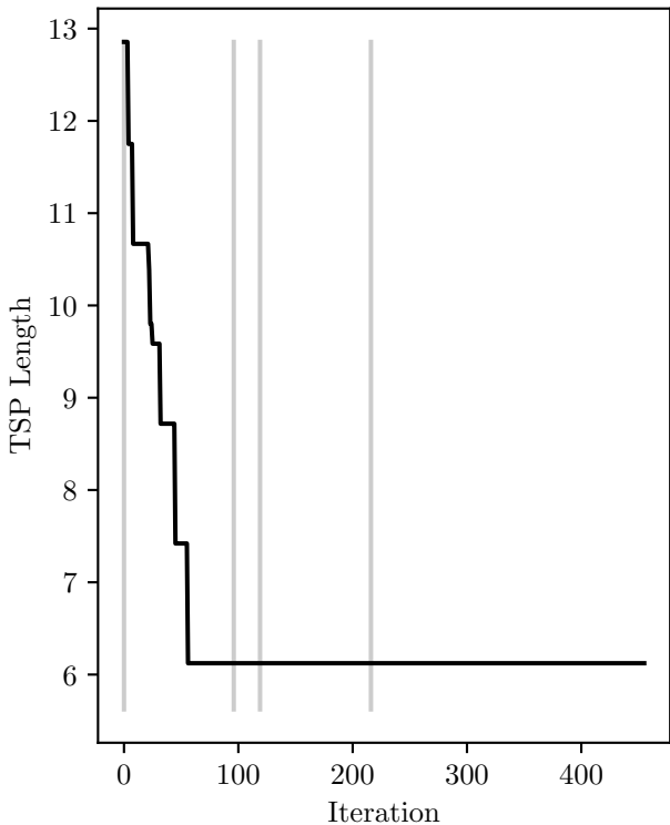
TSP cost evolution, final cost: 6.12
