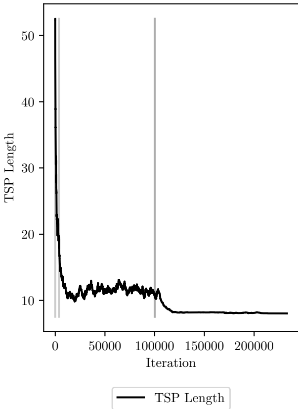
TSP cost evolution, final cost: 8.03
