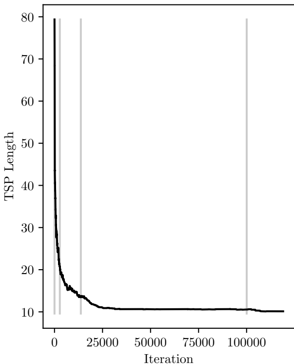
TSP cost evolution, final cost: 10.13
