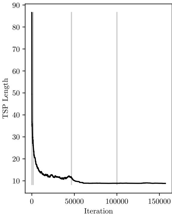
TSP cost evolution, final cost: 8.84
