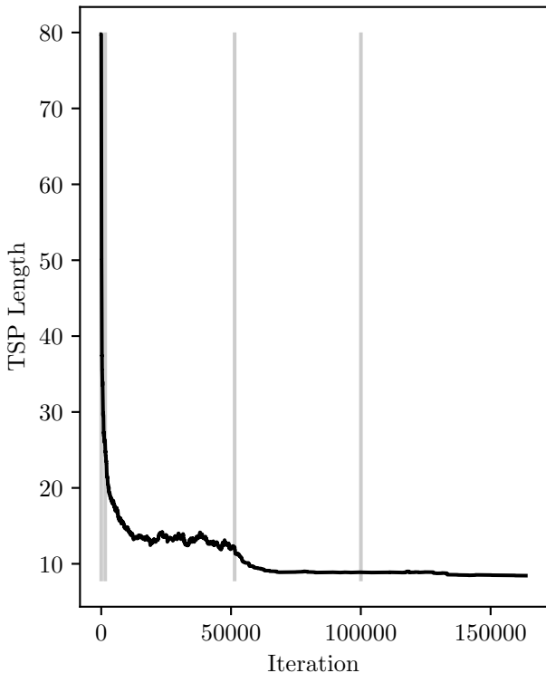
TSP cost evolution, final cost: 8.44
