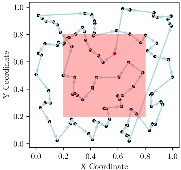
TSP Route, Cost: 9.14
