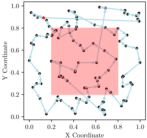
TSP Route, Cost: 14.03
