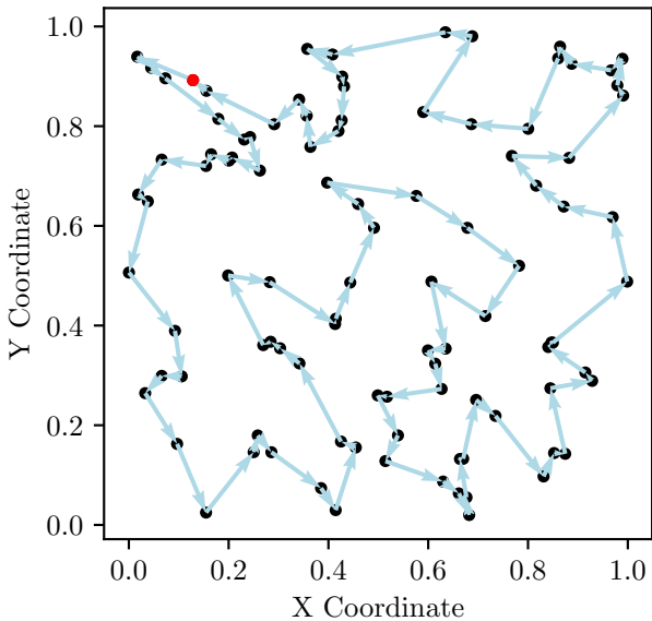
TSP Route, Cost: 8.03
