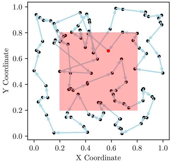
TSP Route, Cost: 10.13
