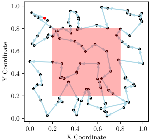
TSP Route, Cost: 8.84
