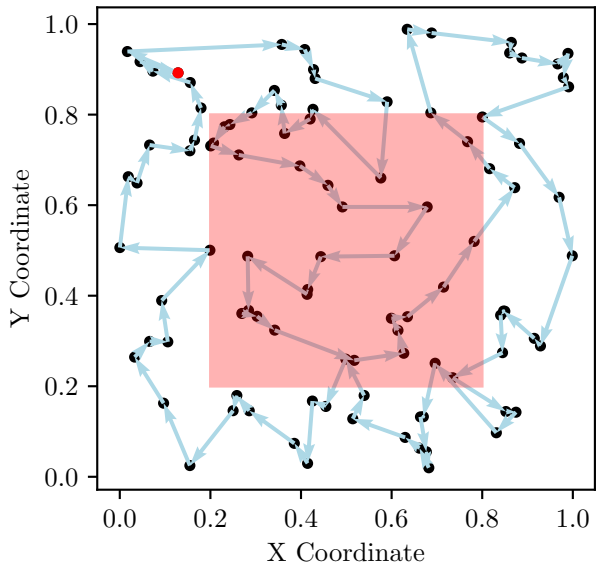
TSP Route, Cost: 8.87
