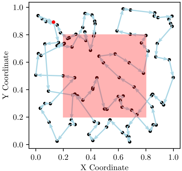
TSP Route, Cost: 9.79
