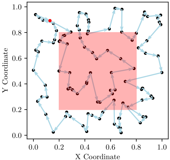
TSP Route, Cost: 8.44
