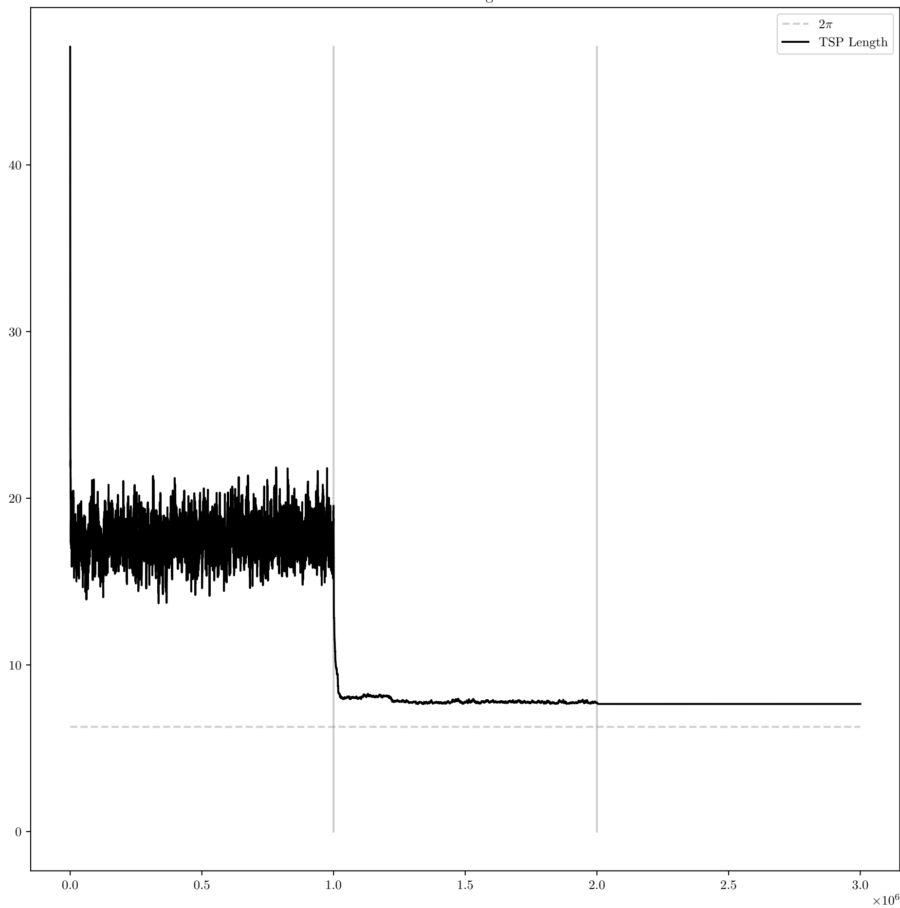
TSP convergence
