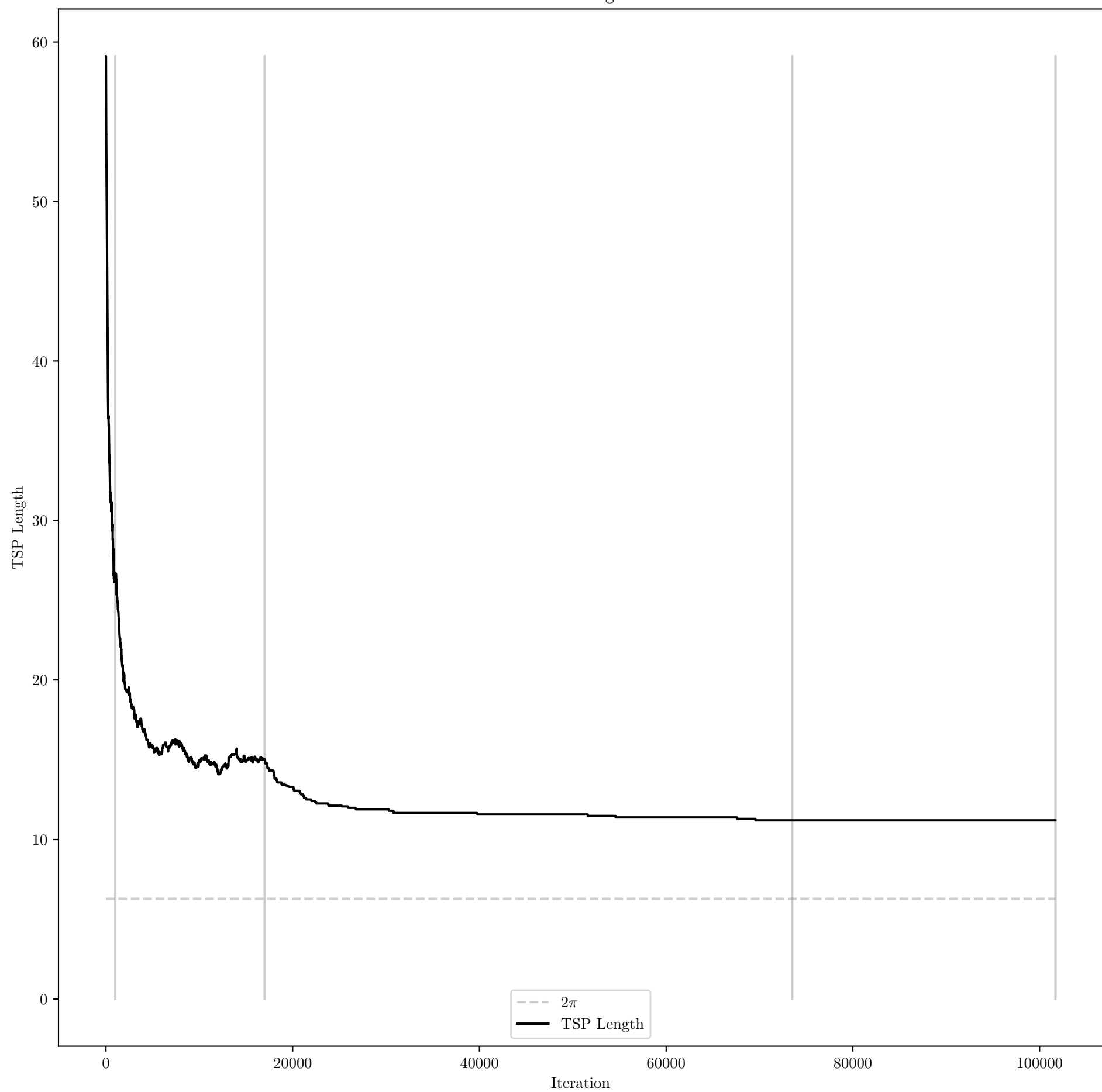
TSP convergence
