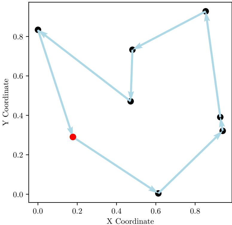
TSP Route, Cost: 3.44
