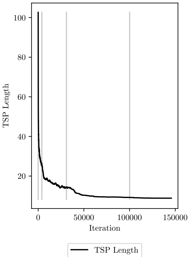
TSP cost evolution, final cost: 8.83
