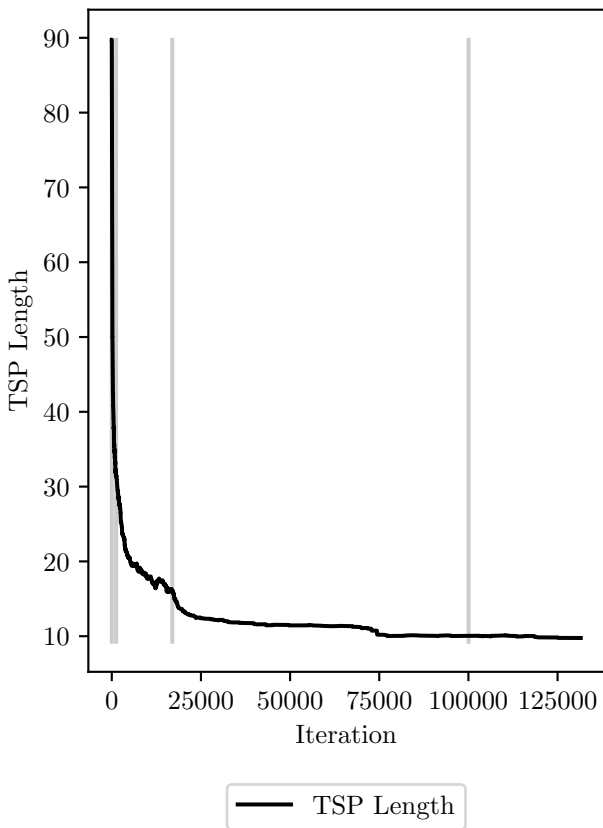
TSP cost evolution, final cost: 9.76
