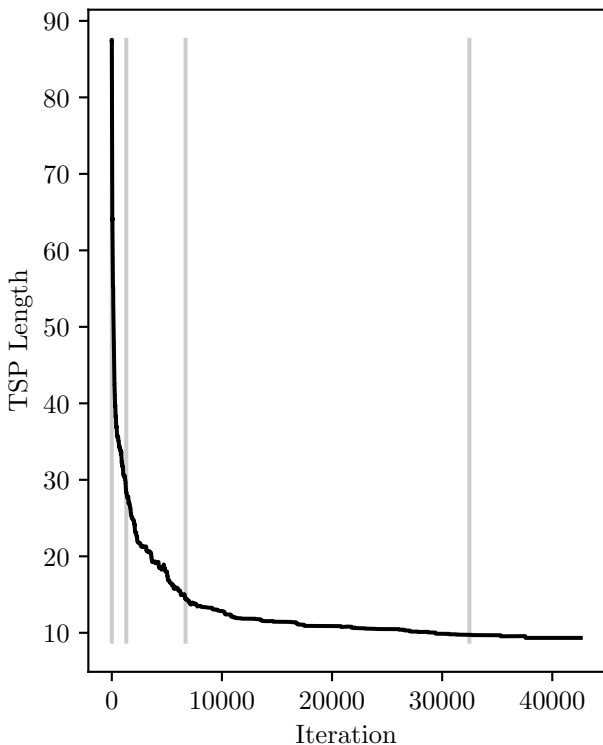
TSP cost evolution, final cost: 9.33
