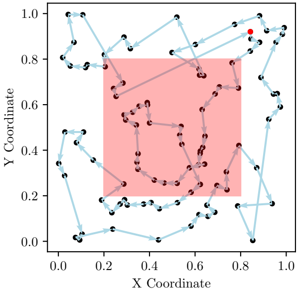
TSP Route, Cost: 12.90
