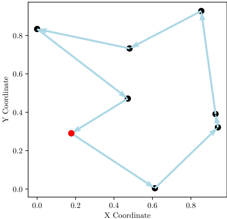
TSP Route, Cost: 3.39
