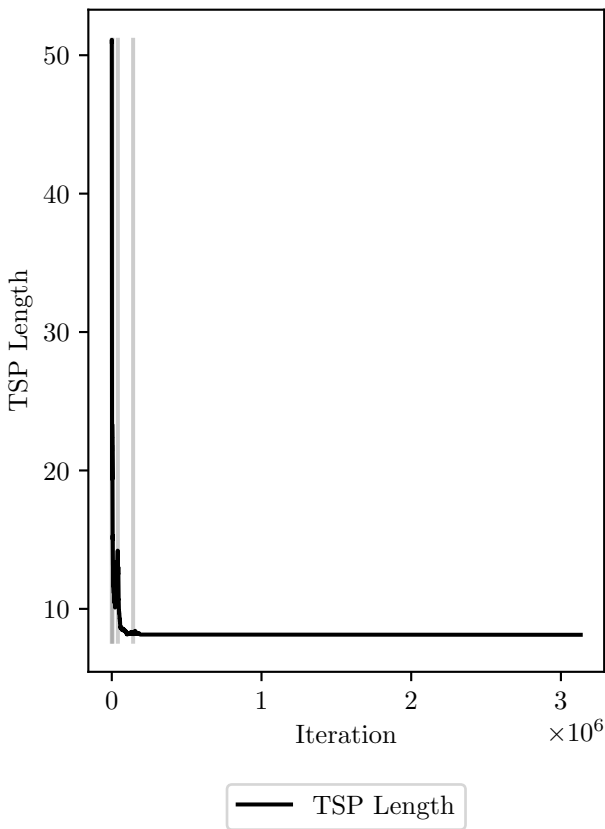
TSP cost evolution, final cost: 8.13
