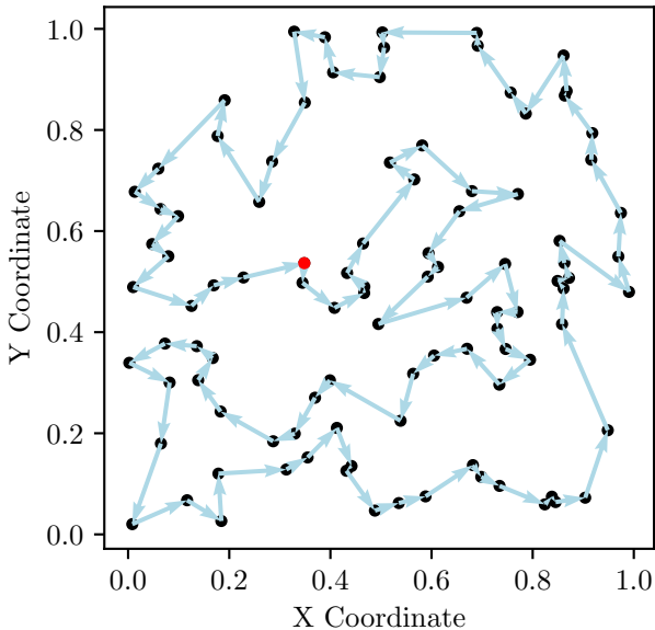
TSP Route, Cost: 8.13
