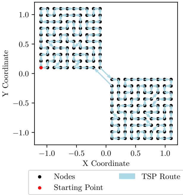
TSP Route, Cost: 23.18
