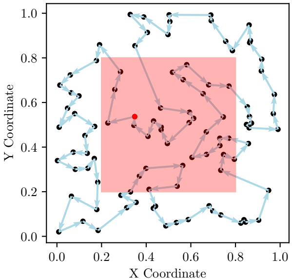
TSP Route, Cost: 8.52
