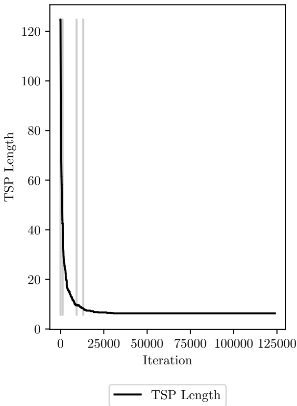
TSP cost evolution, final cost: 6.28
