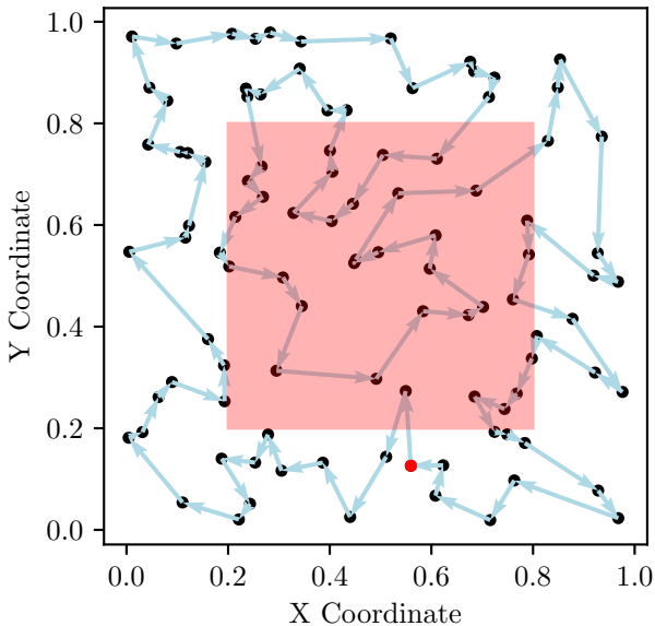
TSP Route, Cost: 9.09
