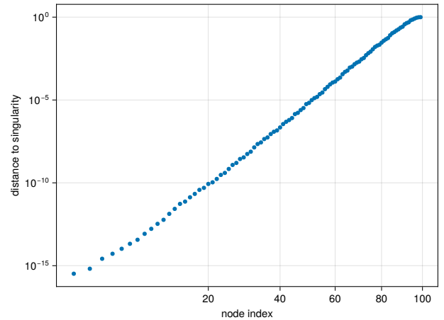
Fig. 4: Positive nodes selected by continuum AAA for the function |x| over [-1, 1] . They cluster near the singularity at x = 0 .
