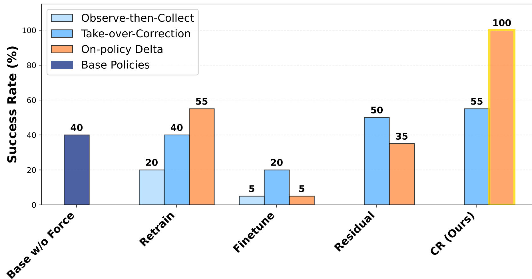
Gear Insertion
