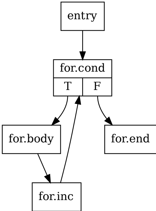
CFG for 'foo' function
