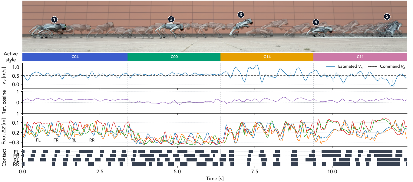
Fig. 3. Style switching on hardware under a fixed task command. Deployment of the CODES policy on the Unitree Go2 at a constant 0.5 m/s forward command with zero lateral and yaw-rate components, while the selected reference switches among C04, C00, C14, and C11. The colored band indicates the active style, and dashed lines the switch instants. The policy, reference bank, and state estimation run onboard, without external motion capture or offboard inference. The top row shows a time-lapse composite of the traversal, with numbered markers at successive instants of the run. The panels below report, from top to bottom, the estimated and commanded forward velocity v_x ; the reference consensus cosine of Eq. (21) with respect to the active reference; the base-relative height \Delta z of the four feet (FL, FR, RL, RR); and the kinematically inferred contact states. The command is identical across all four segments, while foot-swing amplitude, contact timing, and base posture differ, indicating that the reference changes how the command is executed rather than which command is tracked. Videos of the hardware execution are provided on the project website.
