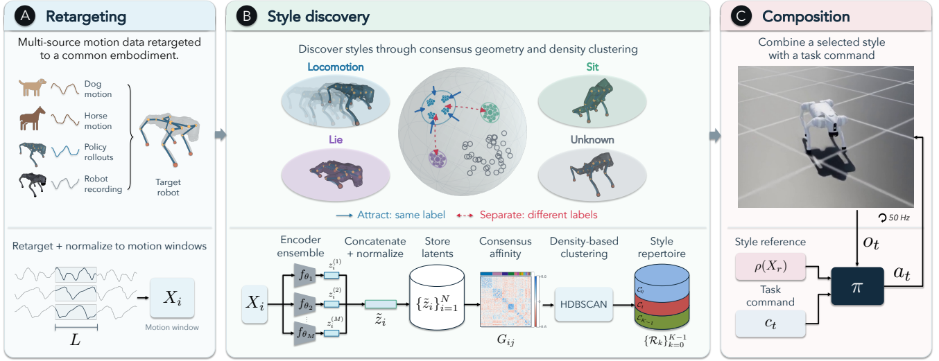
Fig. 1. Learning and composing motion styles for quadruped control. (A) Motions are retargeted to a common representation compatible with the robot’s kinodynamics; (B) a weakly-supervised method based on consensus affinity and HDBSCAN identifies a style repertoire; and (C) a policy trained with reinforcement learning composes a style reference from the repertoire and an independent task command for robot control. This makes recorded motion characteristics available under independently selected commands.
