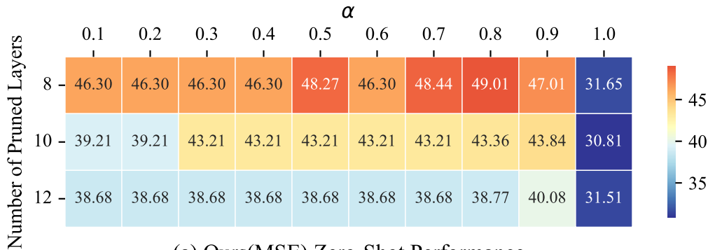
(a) Ours(MSE) Zero-Shot Performance
