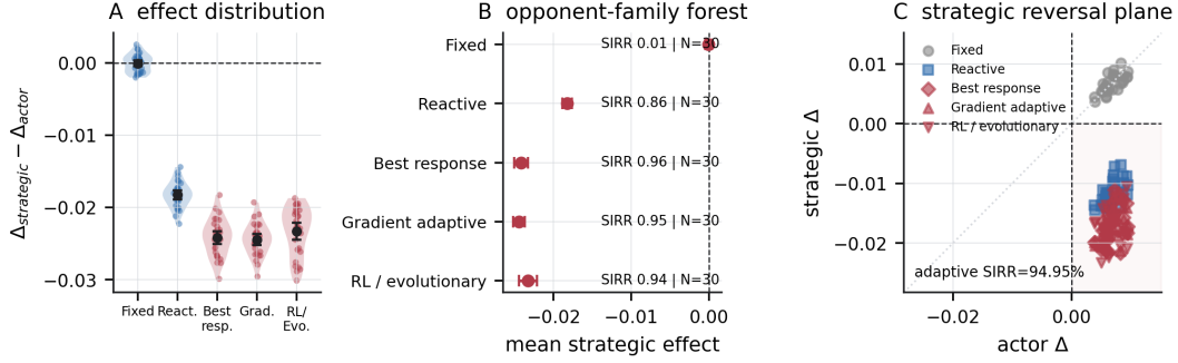
Figure 9: Strategic generalization across opponent mechanisms. Raincloud and forest views show cluster effects and SIRR; the reversal plane uses both color and marker shape so the failure is legible in grayscale.
