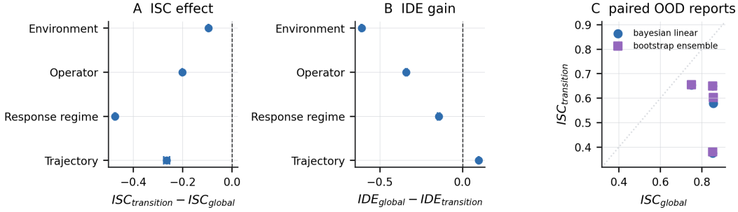
Figure 7: Powered OOD null. Forest intervals are descriptive spans across the two fitted model families in each split; the scatter retains the paired reports and the diagonal indicates equal ISC.
