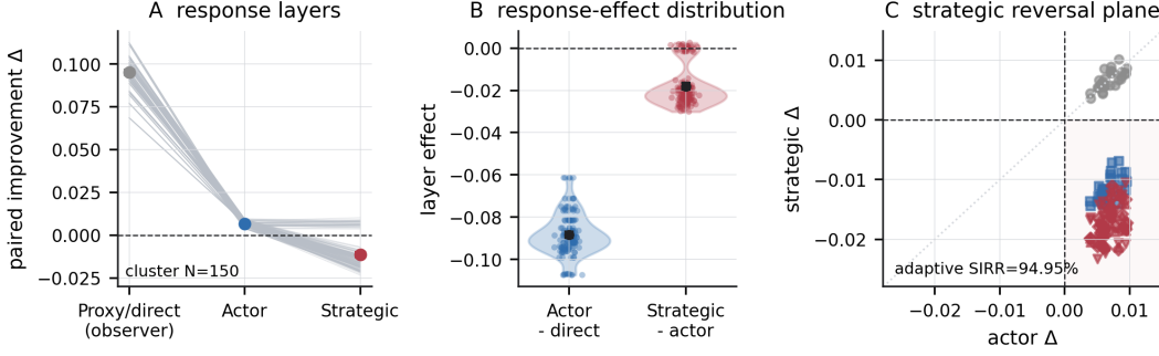
Figure 6: World-response decomposition. Panel A traces paired cluster transitions through proxy/direct observer, actor, and strategic worlds; Panel B separates mechanical and strategic effects; Panel C marks the strategic reversal quadrant.
