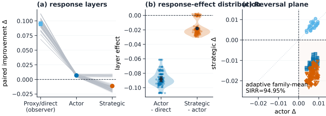
Figure 5: World-response decomposition. Panel a traces 150 family-by-seed observations (five opponent families \times 30 matched seeds) through direct, actor, and strategic worlds; summary intervals use the 30 matched seeds. Panel b separates mechanical and strategic effects; panel c marks the strategic reversal quadrant.
