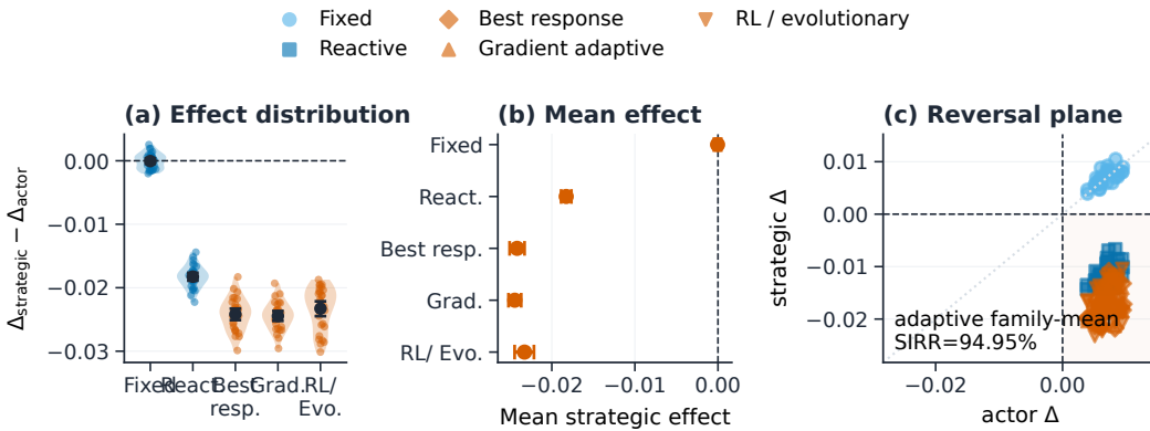
Figure 6: Strategic generalization across opponent mechanisms. Raincloud and forest views show family-specific effects over 30 matched opponent-seed clusters. The reversal plane labels the unweighted mean across the three adaptive families and uses both color and marker shape for grayscale legibility.
