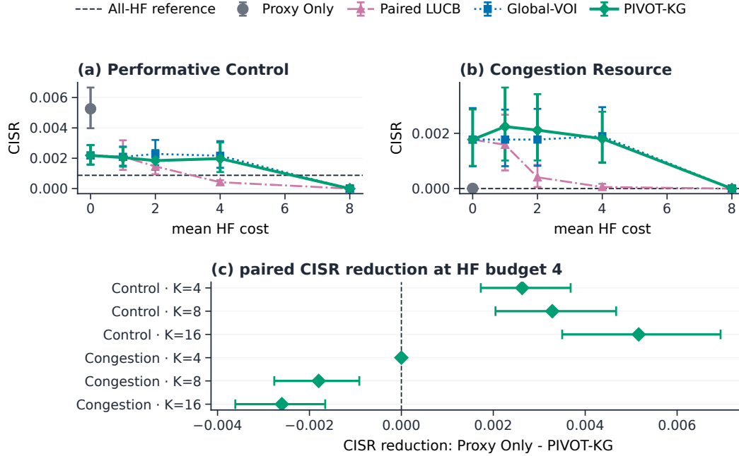
Figure 4: Evidence-efficiency frontier. Matched-cost curves and the fixed-budget forest report selection-regret reduction; the all-HF line is a reference. Intervals are bootstrap intervals over trajectory seeds.
