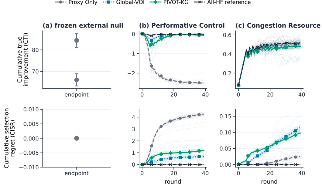
Figure 7: Closed-loop validator outcomes. The top row reports cumulative true improvement (CTI) and the bottom row cumulative improvement-selection regret (CISR); thin curves show seed-level trajectories and markers summarize the compared decision rules.
