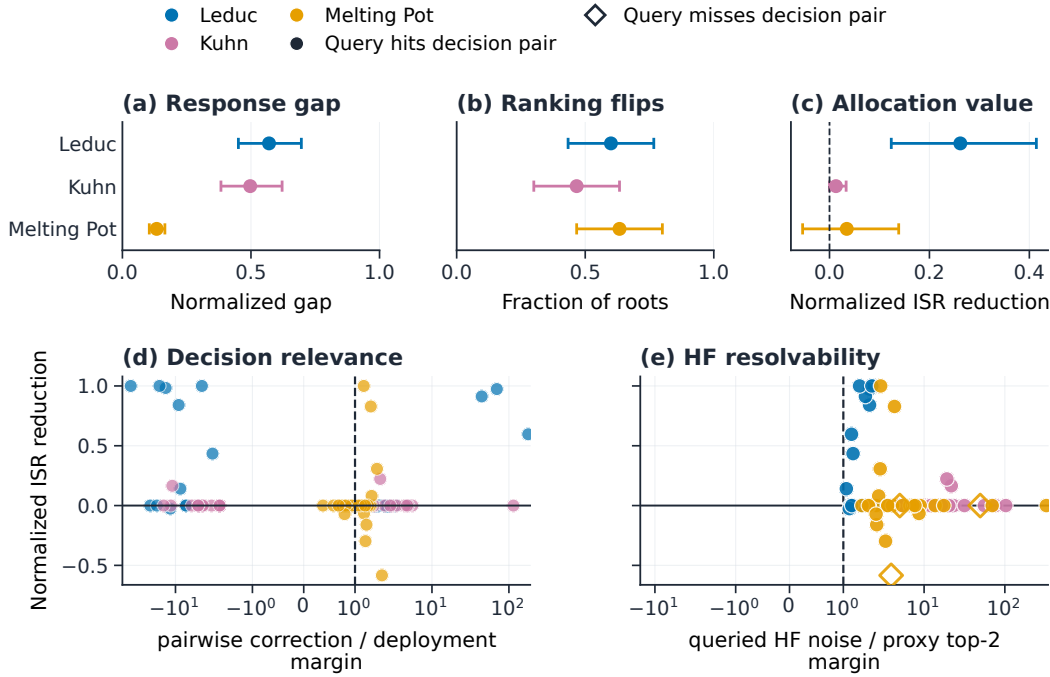
Figure 3: Response magnitude is not allocation value. Panel a reports within-root normalized response gaps; b reports proxy/deployment top-1 flips; c reports normalized ISR reduction; d relates correction-to-margin ratio to normalized ISR reduction; e relates queried HF noise to the proxy top-2 margin. ISR reductions are divided by the within-root deployment range. In e, filled circles denote queries intersecting the ex-post decision-critical pair and open diamonds denote misses.
