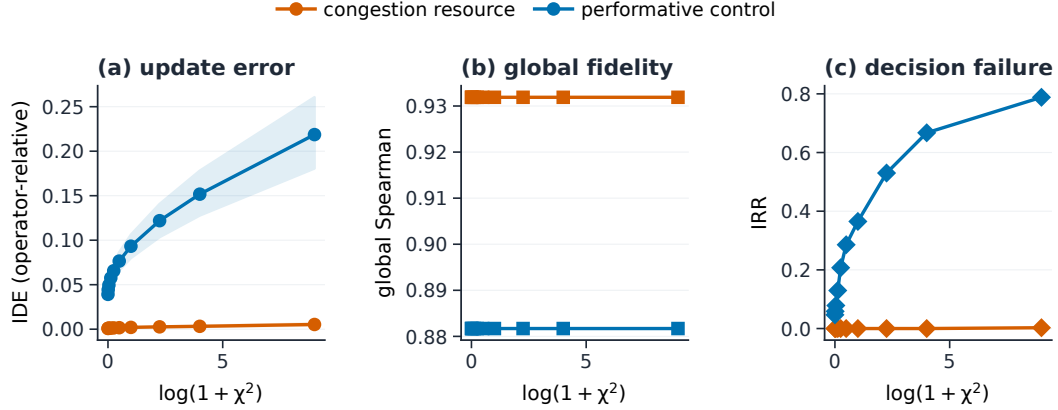
Figure 2: Operator-relative shift diagnostic. Local improvement error rises with registered shift while global policy rank remains comparatively stable. The same environment-by-shift cells show error, rank, and reversal rate.
