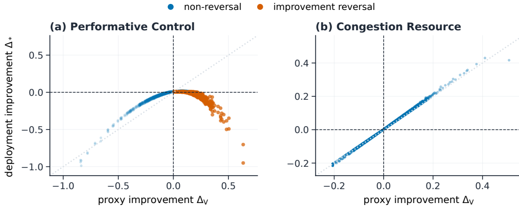
Figure 1: Paired proxy and deployment improvements in the two controlled worlds. The lower-right quadrant is an improvement reversal. Points are a deterministic display subsample; IRR is computed on all transition rows.
