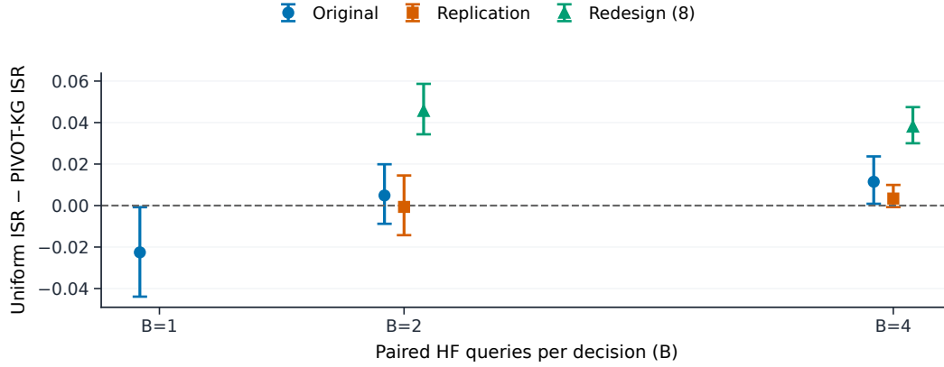
Figure 9: HighwayEnv paired allocation contrasts across the historical, fresh-seed, and eight-candidate redesign cohorts. Positive Uniform-minus-PIVOT ISR favors PIVOT-KG; error bars are paired 95% bootstrap intervals over the registered test seeds.
