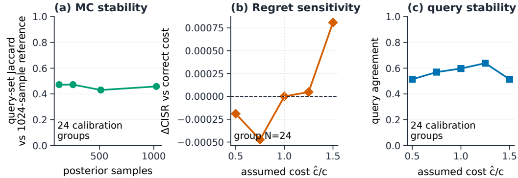
Figure 8: PIVOT-KG sensitivity to posterior sample count and cost misspecification across the registered calibration groups.
