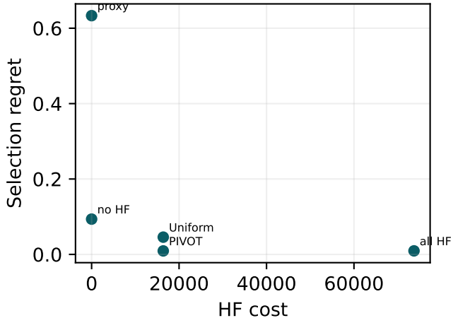
Leduc
