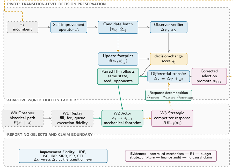
Figure 3: PIVOT validates the replacement operation rather than isolated policy values. A cheap verifier produces proxy improvements and update footprints; a decision-change score selects paired high-fidelity interventions under common state, seed, and opponent conditions. The differential correction ranks candidates for promotion and feeds the next self-improvement round.
