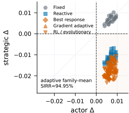
c strategic reversal plane
