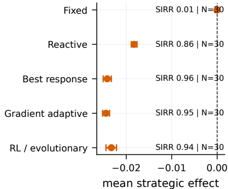
b opponent-family forest
