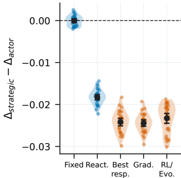
a effect distribution
