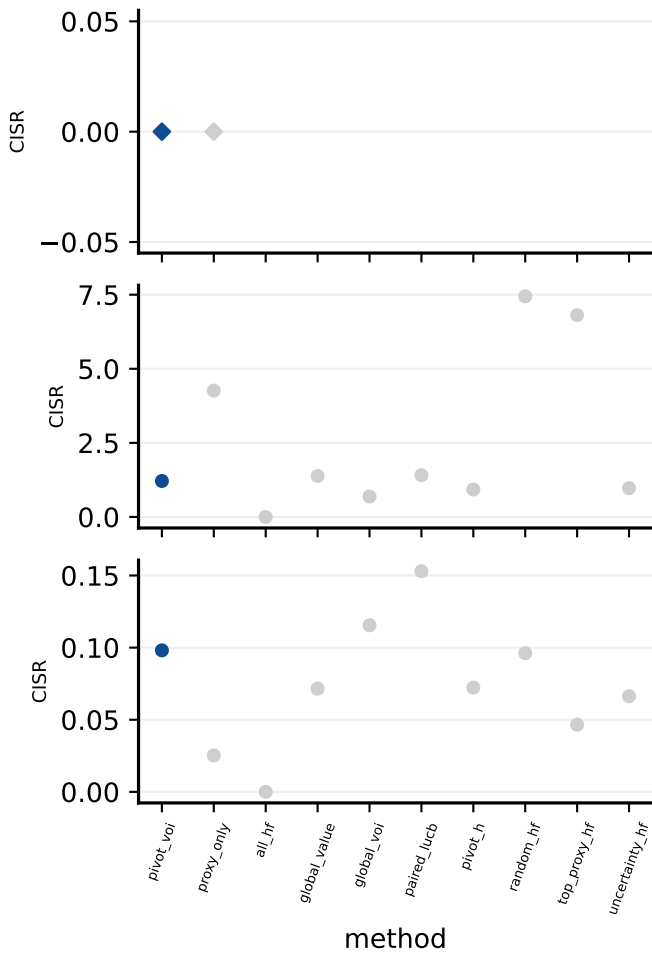
E3C: closed-loop outcomes at matched query budgets
