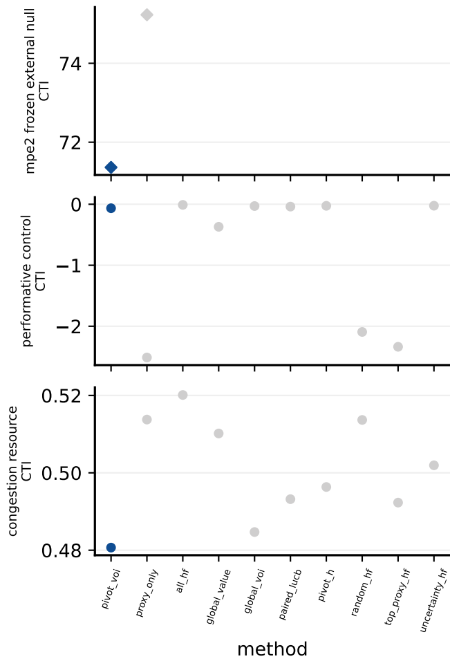
E3C: closed-loop outcomes at matched query budgets
