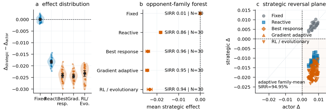
Figure 6: Strategic generalization across opponent mechanisms. Raincloud and forest views show family-specific effects and reversal rates over 30 matched opponent-seed clusters. The reversal plane labels the unweighted mean across the three adaptive families and uses both color and marker shape for grayscale legibility.
