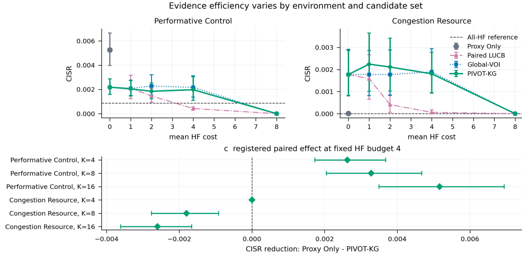
Figure 4: Evidence-efficiency frontier. Matched-cost curves and the fixed-budget forest report selection-regret reduction; the all-HF line is a reference. Intervals are bootstrap intervals over trajectory seeds.
