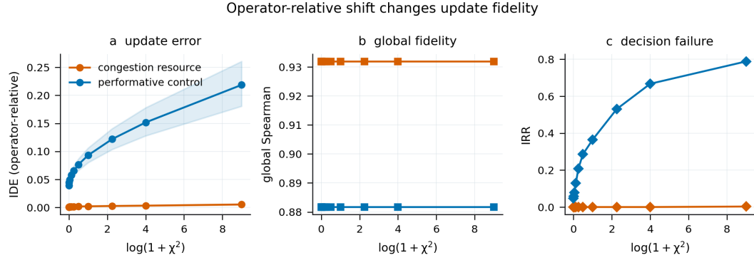
Figure 2: Operator-relative shift diagnostic. Local improvement error rises with registered shift while global policy rank remains comparatively stable. The same environment-by-shift cells show error, rank, and reversal rate.
