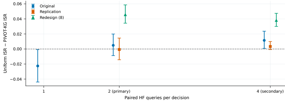
Figure 9: HighwayEnv paired allocation contrasts across the historical, fresh-seed, and eight-candidate redesign cohorts. Positive Uniform-minus-PIVOT ISR favors PIVOT-KG; error bars are paired 95% bootstrap intervals over the registered test seeds.
