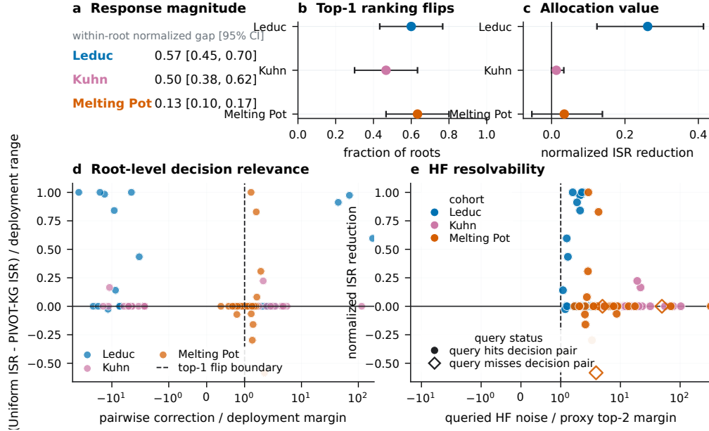
Figure 3: Response magnitude is not allocation value. Panel a reports within-root response gaps; b reports proxy/deployment top-1 flips; c reports normalized ISR reduction; d relates correction-to-margin ratio to normalized gain; e relates queried HF noise to the proxy top-2 margin. Filled circles denote queries intersecting the ex-post decision-critical pair and open diamonds denote misses.
