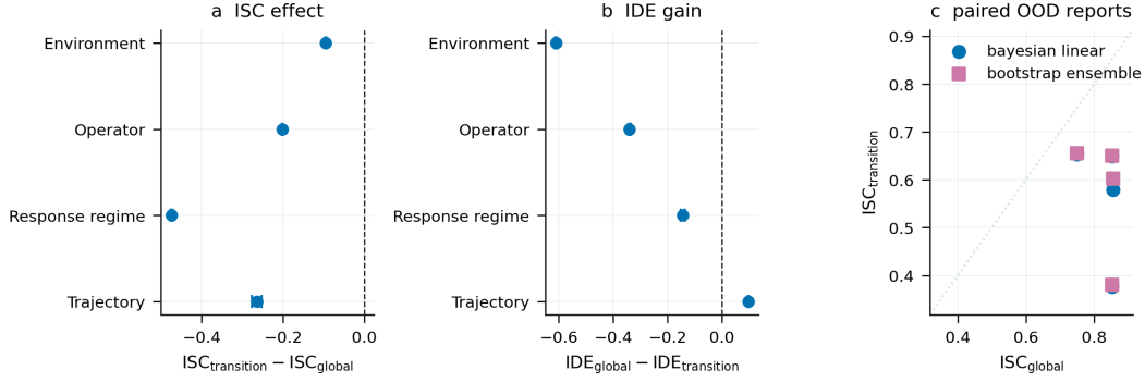
Figure 10: OOD evaluator comparison. Forest horizontal ranges are descriptive spans across the two fitted model families in each split; the scatter retains paired reports and the diagonal indicates equal ISC.
