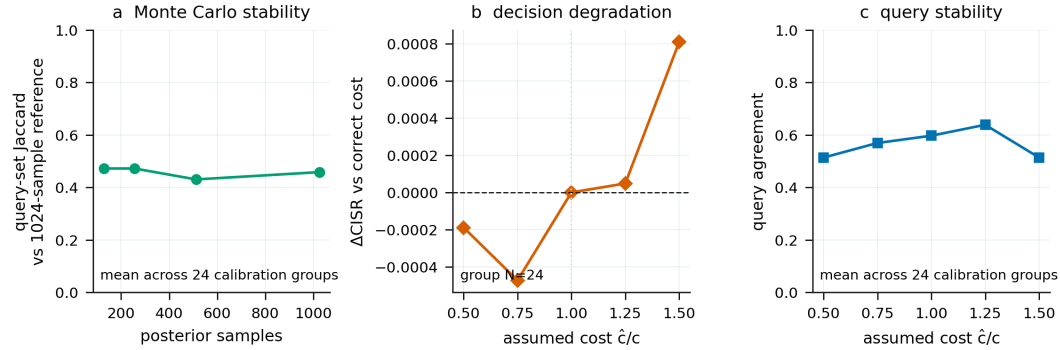
Figure 8: PIVOT-KG sensitivity to posterior sample count and cost misspecification across the registered calibration groups.
