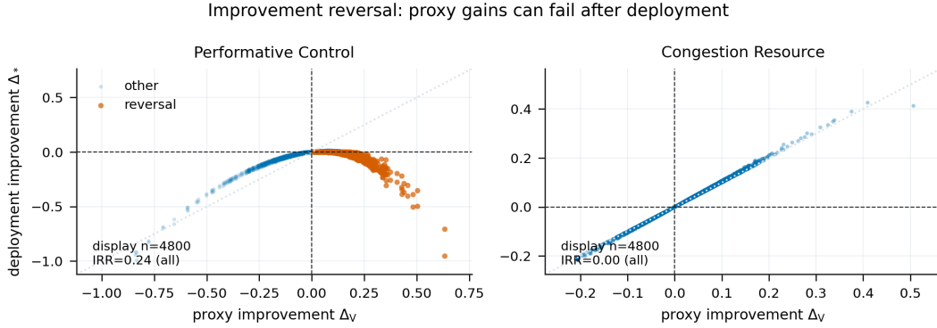
Figure 1: Paired proxy and deployment improvements in the two controlled worlds. The lower-right quadrant is an improvement reversal. Points are a deterministic display subsample; IRR is computed on all transition rows.
