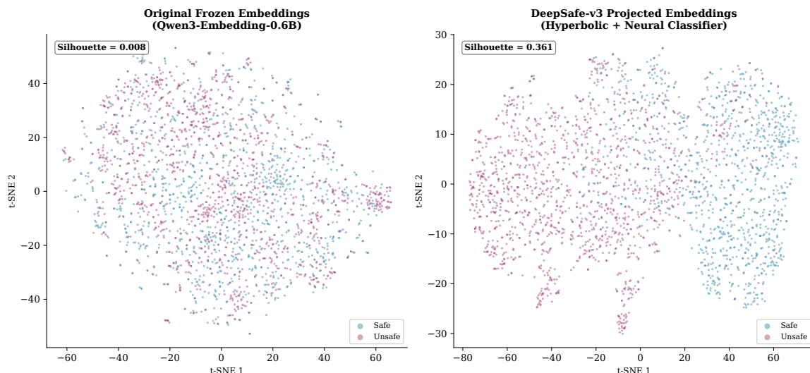
Figure 7: t-SNE visualization of original Qwen3-Embedding-0.6B embeddings (left, 2D silhouette \approx 0.008 ) vs. DeepSafe-projected embeddings (right, 2D silhouette \approx 0.36 ). The projection head learns to structurally separate safe from unsafe content; see §4 for full 256-dimensional silhouette scores.
