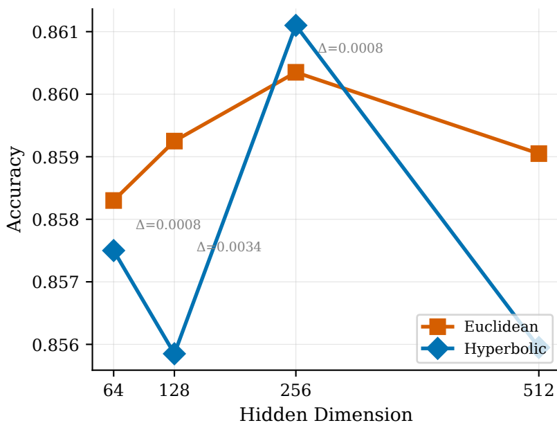
Test Accuracy (BCE-only, no DeepSafe loss)
