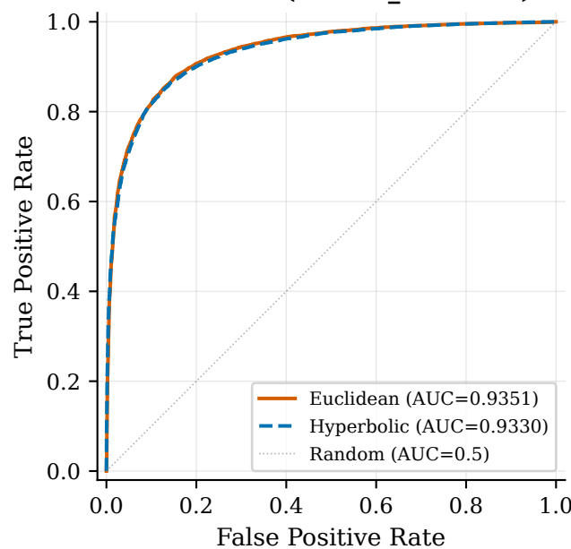
ROC Curve (hidden_dim=256)
