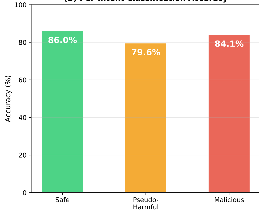
(B) Per-Intent Classification Accuracy
