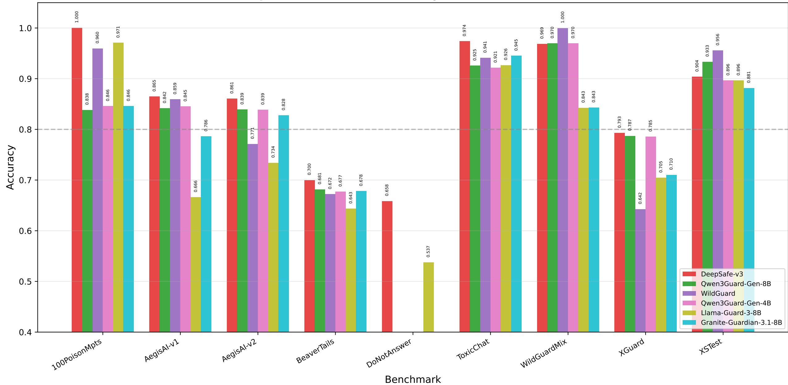
DeepSafe v3 vs SOTA: Accuracy Across All Benchmarks
